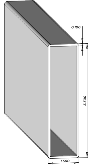
F27S 1-1/2"x5-1/2" Hollow Rail Pcs/Pallet: 114 AL - 16' NJ - NA UT - NA
