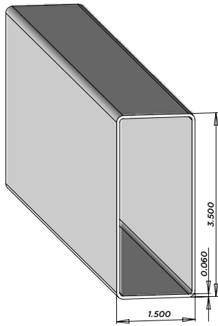
F28S 1-1/2" x 3-1/2" Standard Rail Pcs/Pallet: 182 AL - NA NJ - NA UT - 57-1/2"
