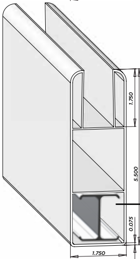
F37C 1-3/4"x5-1/2" Gorilla® Pocket Rail 7/8" x 1 3/4" Deep
