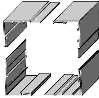
6"x6" Gorilla® Wrap FPW6 Pcs/Box: 4 posts per box Bulk: 74 posts per bundle Length - 10'
