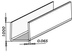
F83S (0.065 Wall) 7/8" U-Channel Standard
