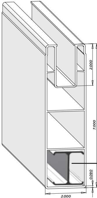
F3BF 2"x 7" Gorilla® Pocket Rail 7/8" x 2" Deep Pcs/Pallet: 66 AL - NA NJ - 94", 95", 16' UT - NA
