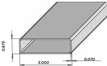
F57C (0.070 Wall) 7/8" X 3" Standard Pickets Pcs/Pallet: 355 AL - 12', 16' NJ - 45-7/8", 12', 16' UT - 16'
