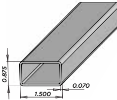
F65S (0.070 Wall) 7/8"x1-1/2" Standard Pickets Pcs/Pallet: 402 AL - 16' NJ - 16' UT - 16'
