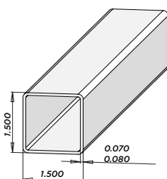
F42H (0.080 Wall) 1-1/2"x1-1/2" Gorilla® Pickets Pcs/Pallet: 450 AL - 16' NJ - NA UT - 16'
