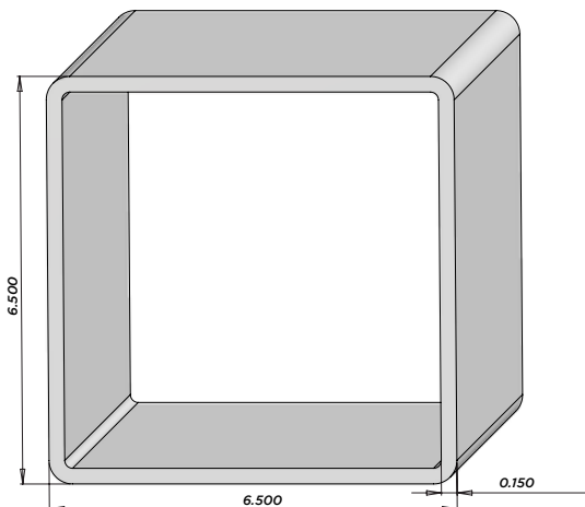
F08E (0.150 wall) 6-1/2"x6-1/2" Post Pcs/Pallet: 49 AL - 9', 16'
