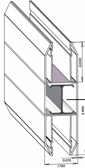
F3PM 1-3/4"x5-1/2" Nexus® Mid-Rail 7/8" x 2" Deep
