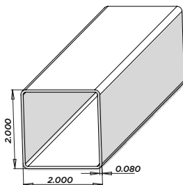
F40S (0.080 Wall) 2"x2" Standard Pickets Pcs/Pallet: 230 AL - 16' NJ - NA UT - NA
