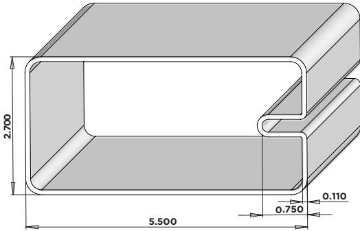
Tuf-Fence® Lattice Top Rail FT13 96.25"
