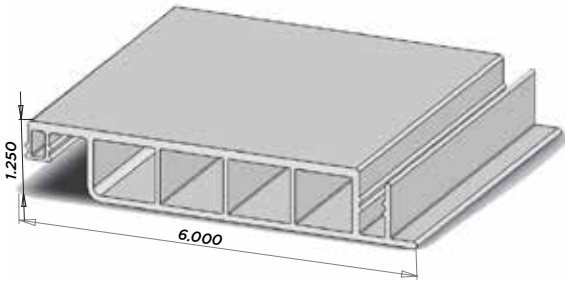
Gorilla Deck® G3 F70E Patent #6,324,796 Pcs/Pallet: 49 AL - 16', 20', 24'
