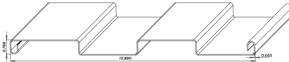
F55B (0.055 wall) 7/8" x 14" Privacy No Emboss Panel Pcs/Pallet: 96 AL - 29", 64", 12'6" NJ - NA UT - NA
