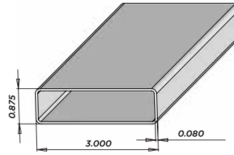
F57H (0.080 Wall) 7/8" X 3" Gorilla® Pickets
