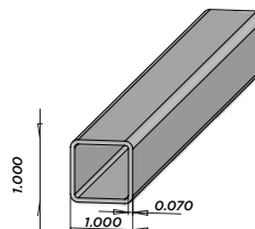
F45S (0.070 Wall) 1"x1" Standard Pickets Pcs/Pallet: 450 AL - 16' NJ - NA UT - 16'
