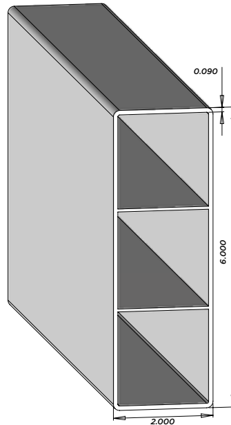
F22C 2"x6" Ribbed Rail Pcs/Pallet: 88 AL - 8', 12', 16' NJ - 16' UT - 12', 16', 24'
