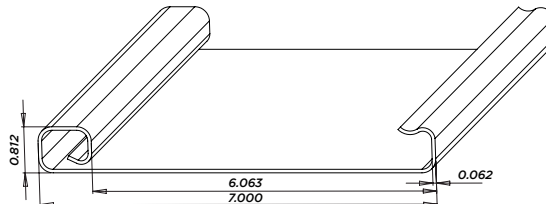
F55N (0.062 wall) 7/8" x 6" Privacy Snap Panel Pcs/Pallet: 312 AL - 62-1/4", 16' NJ - NA UT - NA
