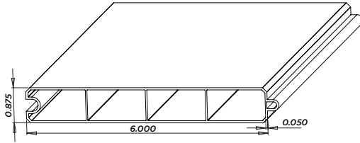
F54U (0.050 Wall) 7/8"x6" T&G Utility
