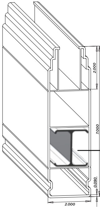
F3P2 2"x7" Nexus® Pocket Rail 7/8" x 2" Deep - Patent Pending Pcs/Pallet: 66 AL - 71-1/2", 94", 16' NJ - NA UT - NA
