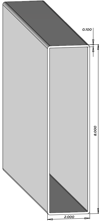
F20S 2" X 8" Hollow Rail Pcs/Pallet: 66 AL - 16', 24' NJ - NA UT - 16' 24'
