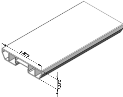
Gorilla® Lock Deck F71A Patent #6,594,961 Pcs/Pallet: 49 AL - 16', 20', 24'
