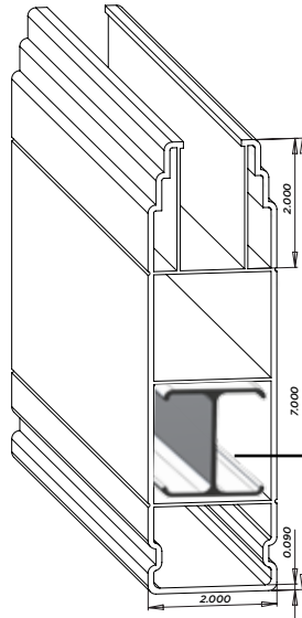
F3P2 2"x7" Nexus® Pocket Rail 7/8" x 2" Deep
