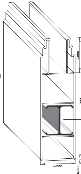
F31S 2"x7" Railmaster 1" Pocket Rail 1" x 1 3/4" Deep Pcs/Pallet: 79 AL - NA NJ - NA UT - 8', 16'
