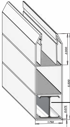
F3P5 1-3/4"x5-1/2" Nexus® Pocket Rail 7/8" x 2" Deep
