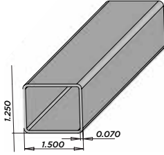
F47S (0.070 Wall) 1-1/4"x1-1/2" Standard Pickets Pcs/Pallet: 510 AL - 16' NJ - NA UT - NA
