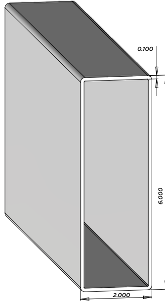
F22E 2"x6" Hollow Rail Pcs/Pallet: 88 AL - 12', 16', 24' NJ - NA UT - 12', 16', 24'
