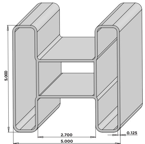
Tuf-Fence® Mid-Rail FT11 96.25"
