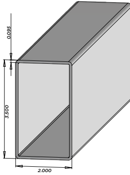
F24E (0.095 Wall) 2"x3-1/2" Hollow Standard Rail (ER1 - AL only)
