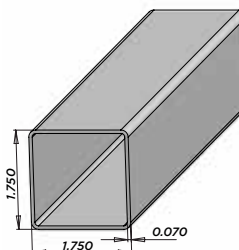
F41S (0.070 Wall) 1-3/4"x1-3/4" Standard Pickets Pcs/Pallet: 312 AL - 16' NJ - NA UT - 16'
