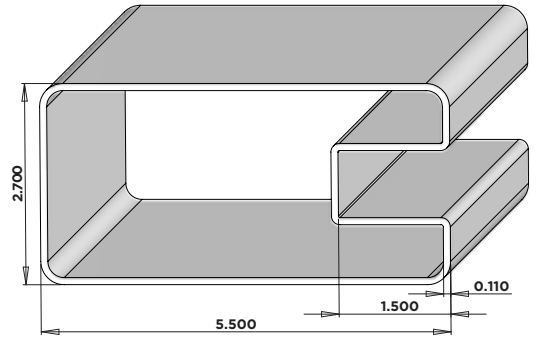
Tuf-Fence® Pocket Rail FT12 96.25"
