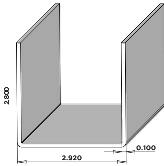
Tuf-Fence® U-Channel (Long Leg) FT03 6', 8'
