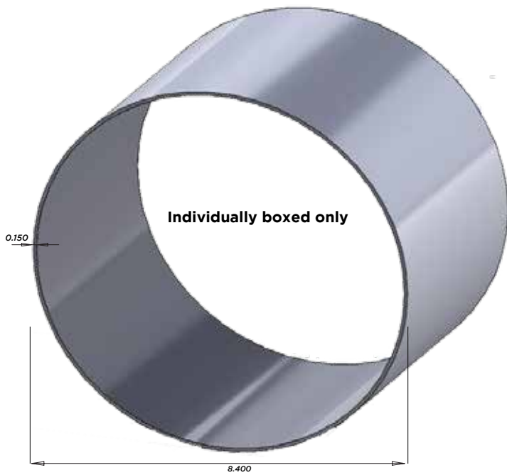
TD84 (0.150 wall) 8.40" Round Column Pcs/Box: 1 Boxes/Skid: 10 SOLD IN SKID QUANTITIES ONLY AL - 9'
