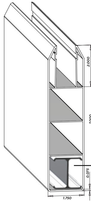
F3P2 2"x7" Nexus® Pocket Rail 7/8" x 2" Deep - Patent Pending Pcs/Pallet: 66 AL - 71-1/2", 94", 16' NJ - NA UT - NA
