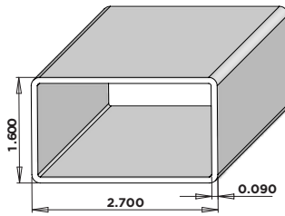
Tuf-Fence® Insert for H-Post FT02 8'
