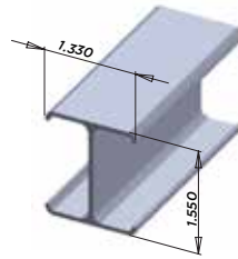
1-1/2" x 5-1/2" Gorilla® Pocket Rail Insert G32GP093-06505
