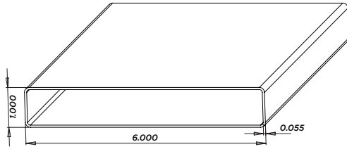
F53S (0.055 wall) 1"x6" Hollow Utility Pcs/Pallet: 176 AL - NA NJ - NA UT - 16'
