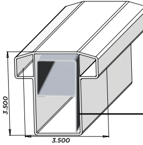
F35C (0.090 Wall) 3-1/2" Gorilla® T-Rail (ER1 - AL only)
