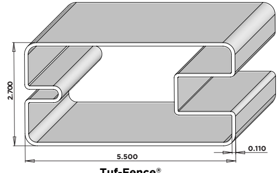
Tuf-Fence® Mid-Rail FT11 96.25"
