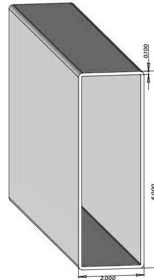
F22E 2"x6" Hollow Rail
