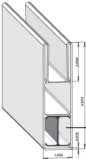
F32G 1-1/2"x5-1/2" Gorilla® Pocket Rail 7/8" x 2" Deep
