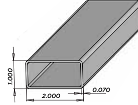
F48S (0.070 Wall) 1"x2" Standard Pickets Pcs/Pallet: 270 AL - 16' NJ - NA UT - 16'
