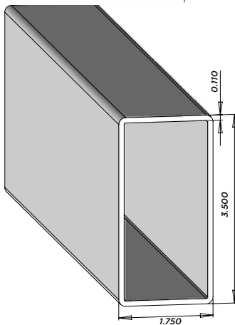
F25B (0.110 Wall) 1-3/4" x 3-1/2" Hollow Standard Rail
