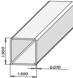
F42S (0.070 Wall) 1-1/2"x1-1/2" Standard Pickets (ER1 - AL only)
