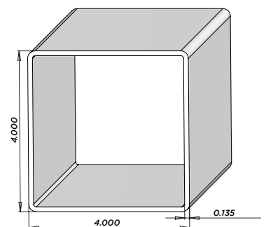
F12N (0.135 wall) 4"x4" Standard Post
