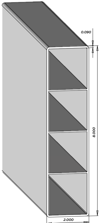
F20R 2"x8" Ribbed Rail Pcs/Pallet: 66 AL - 16', 24' NJ - NA UT - NA
