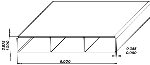
F53U (0.080 wall) 1"x6" Utility Ribbed Pcs/Pallet: 176 AL - NA NJ - NA UT - 16'
