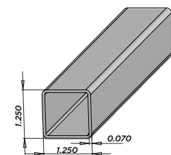
F44S (0.070 Wall) 1-1/4"x1-1/4" Standard Pickets Pcs/Pallet: 350 AL - 16', 32" (1225/pallet) NJ - NA UT - 16'
