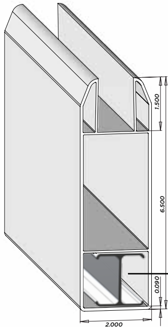
F31S 2"x7" Railmaster 1" Pocket Rail 1" x 1 3/4" Deep Pcs/Pallet: 79 AL - NA NJ - NA UT - 8', 16'
