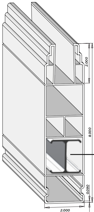
F3P8 2"x8" Nexus® Pocket Rail 7/8" x 2" Deep - Patent Pending Pcs/Pallet: 55 AL - 82-1/2", 94" NJ - NA UT - NA
