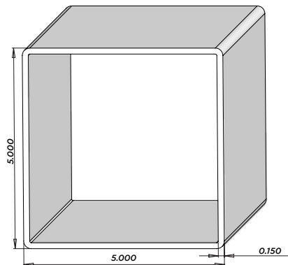
F10C (0.150 wall) 5"x5" Standard Post
