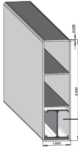
F27C (0.095 Wall) 1-1/2"x5-1/2" Ribbed Rail
