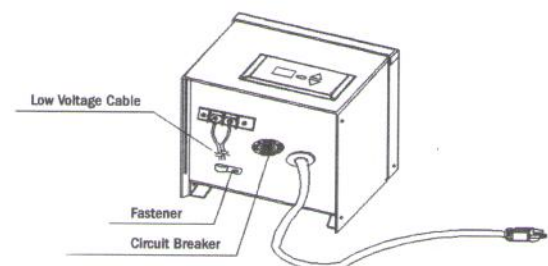
DIAGRAM 3
