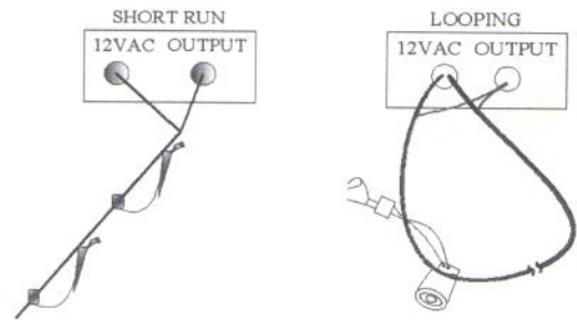
DIAGRAM 3B
